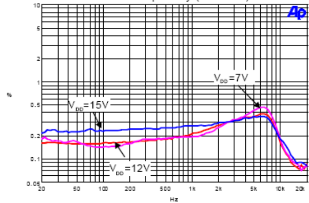
11. THD+N vs Frequency ( P_o=1\text{W} )
