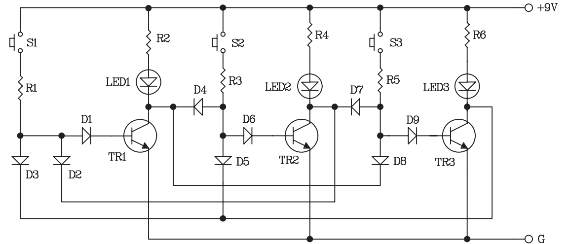
Figure 2. The priority testing game circuit
