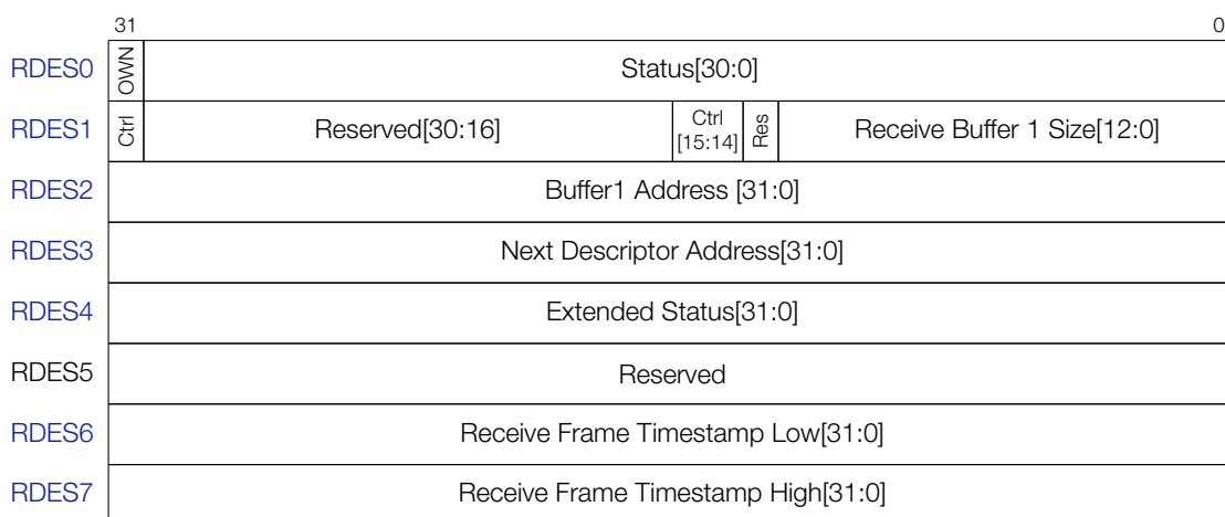
Figure 10-8. Receive Descriptor
