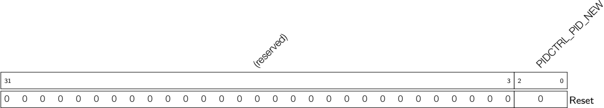
Register 28.13. PIDCTRL_PID_NEW_REG (0x048)
