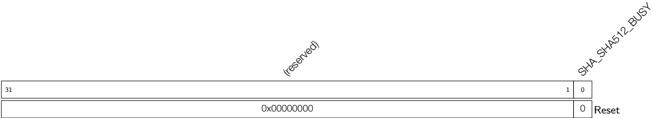
Register 23.17. SHA_SHA512_BUSY_REG (0x0BC)
