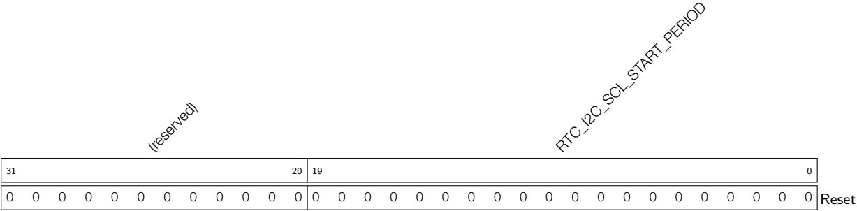
Register 30.18. RTC_I2C_SCL_START_PERIOD_REG (0x040)
