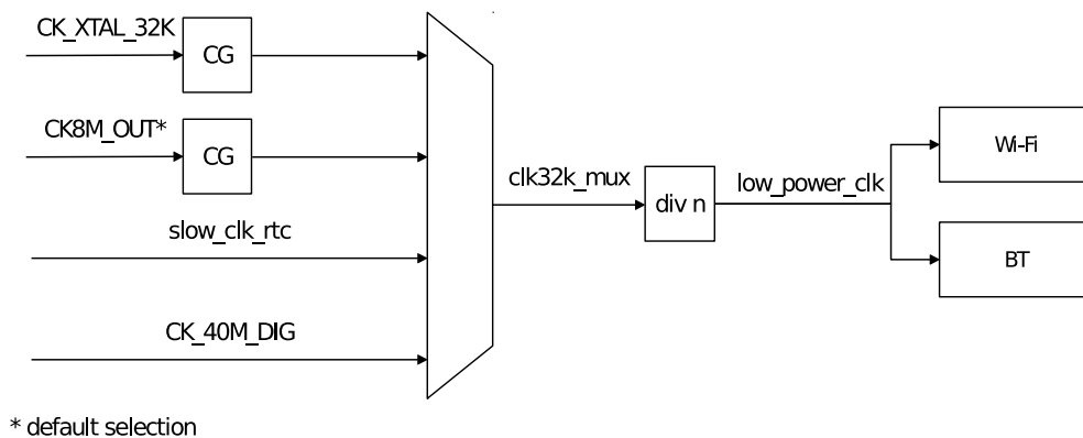
Figure 31-8. Digital Low-Power Clocks
