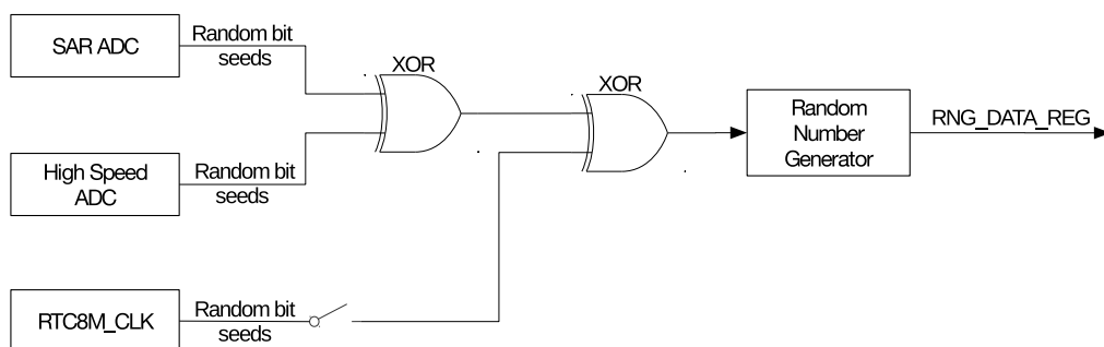
Figure 25-1. Noise Source
