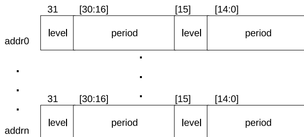
Figure 15-2. Data Structure
