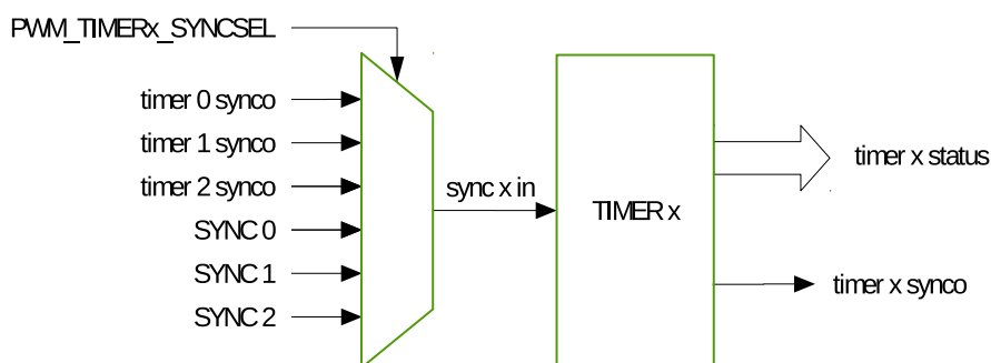
Figure 16-3. Timer Submodule
