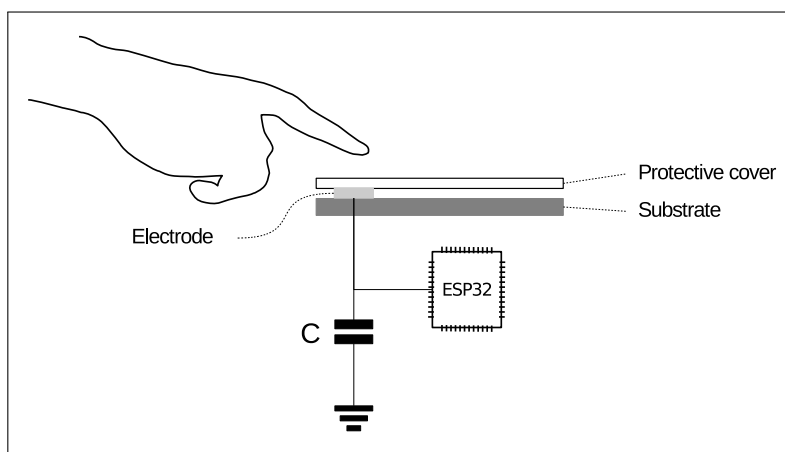
Figure 29-1. Touch Sensor
