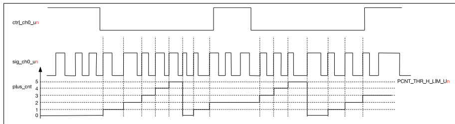
Figure 17-2. PULSE_CNT Upcounting Diagram
