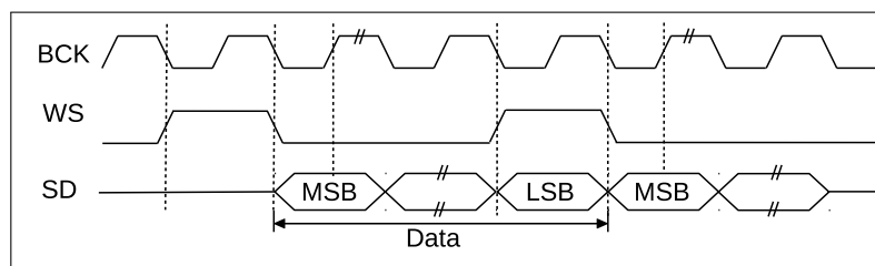
Figure 12-5. PCM Standard
