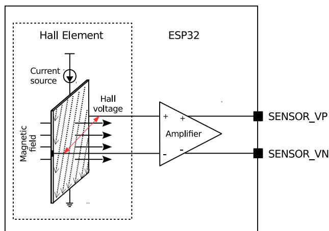
Figure 29-9. Hall Sensor
