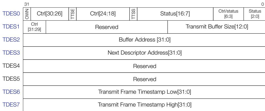
Figure 10-7. Transmit Descriptor
