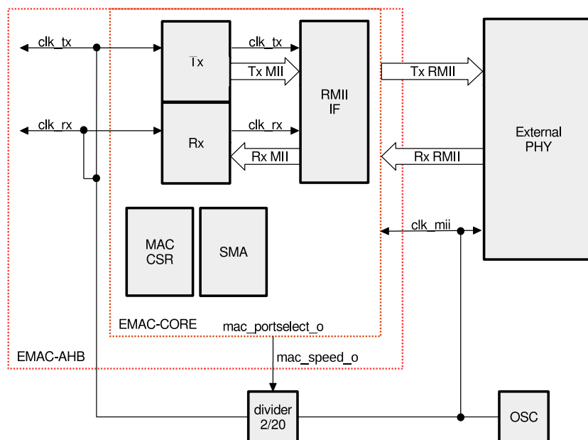
Figure 10-6. RMI Clock
