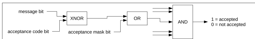
Figure 21-7. Acceptance Filter
