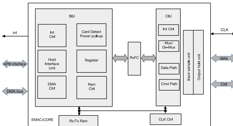
Figure 9-3. SDIO Host Block Diagram
