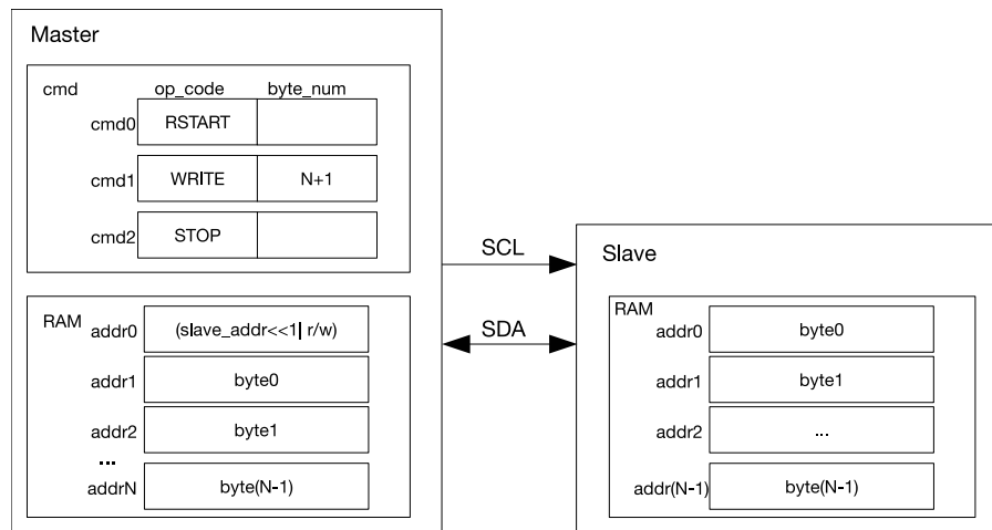
Figure 11-5. I2C Master Writes to Slave with 7-bit Address
