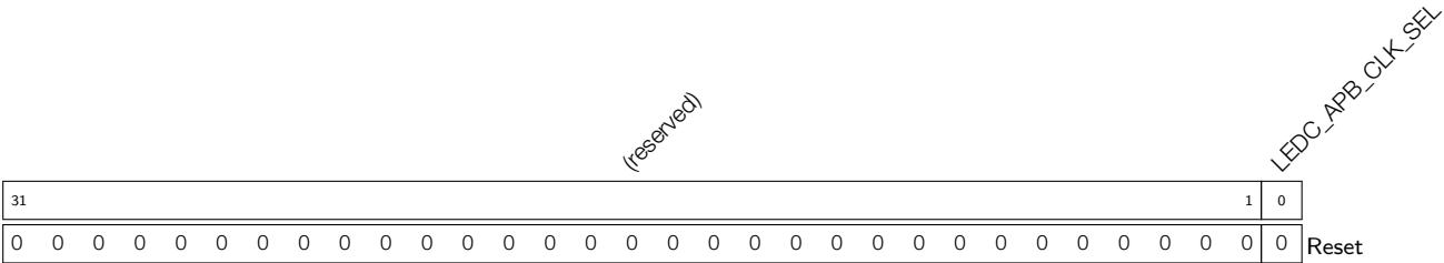
Register 14.19. LEDC_CONF_REG (0x0190)
