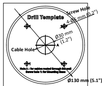
Figure 2-10 Drill Template
