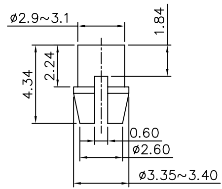
Detail X
