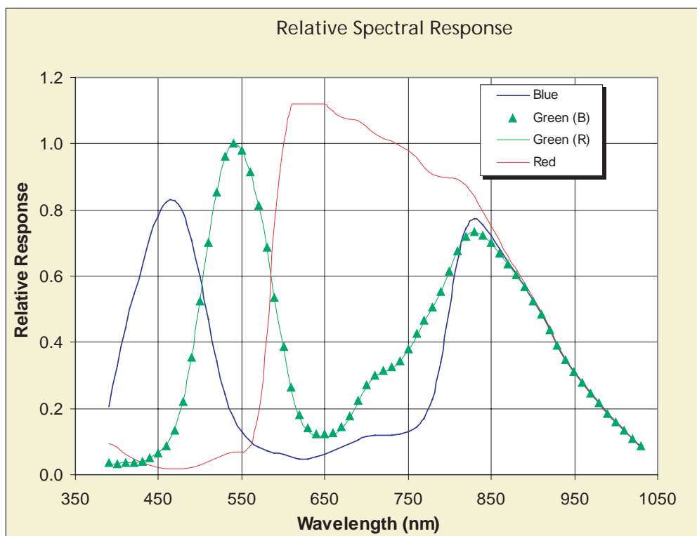
Figure 28: Spectral Response
