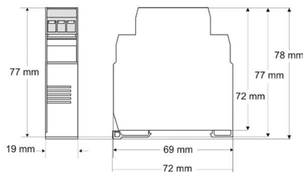
Figure 3 – Dimensions
