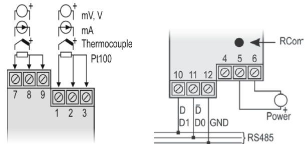
Figure 1 – Electrical Connections
