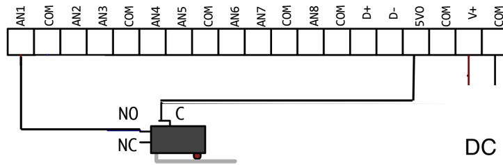
Figure 3 - Wiring a dry contact switch
